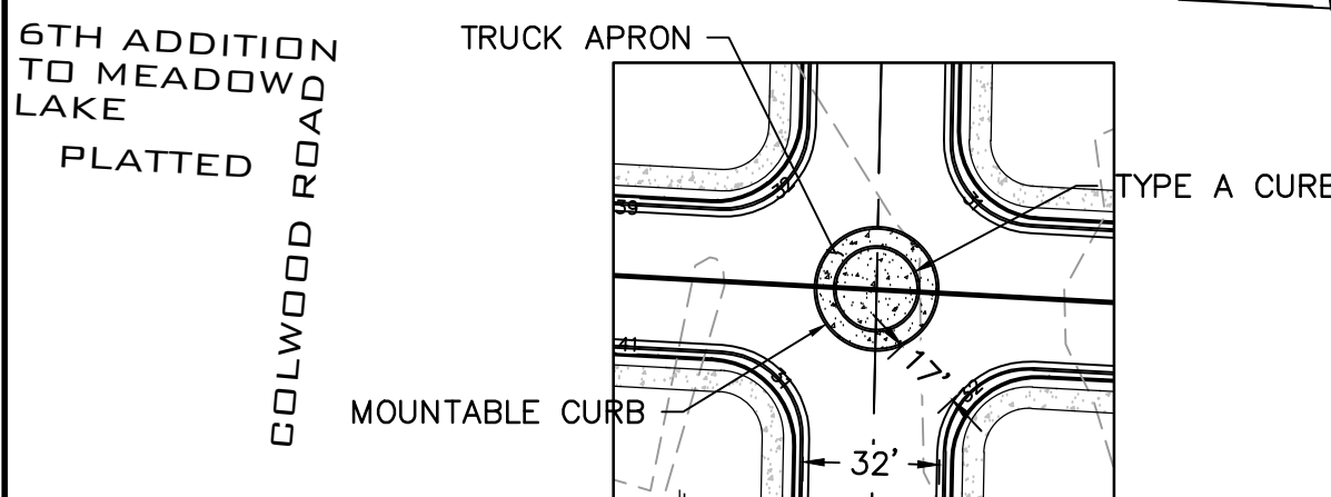
TYPICAL TRAFFIC CIRCLE NOT TO SCALE
