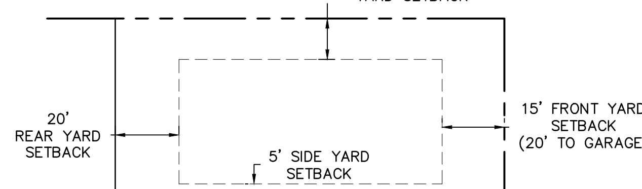
TYP LOT SETBACK DETAIL NOT TO SCALE
